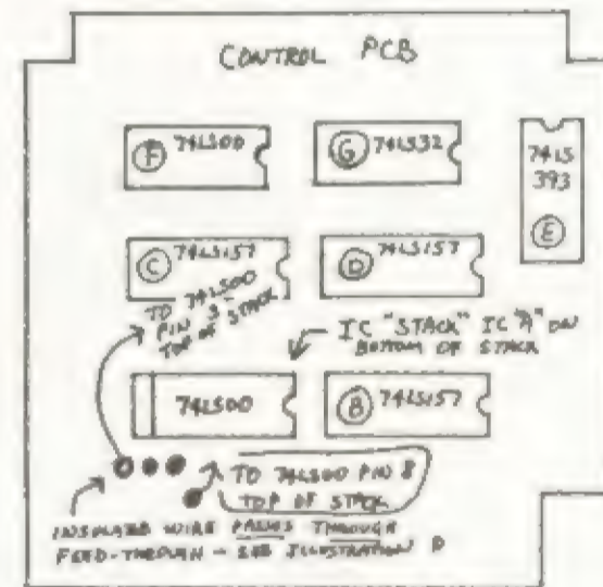
Illustration G: Pad/Feed-Through Locations
